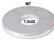
M7, washer largely, 7,5x22mm, 2mm heavily.
